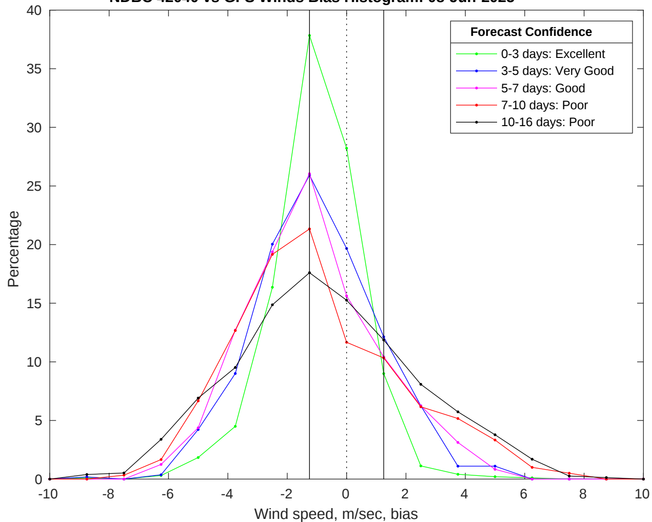
NDBC 42040 vs GFS Winds Bias Histogram: 08-Jun-2025
