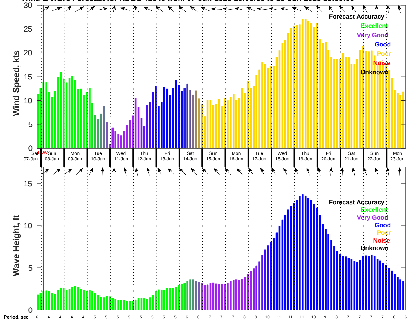
Wind & Wave Forecast for NDBC 42040 from 07-Jun-2025 19:00:00 to 23-Jun-2025 19:00:00
