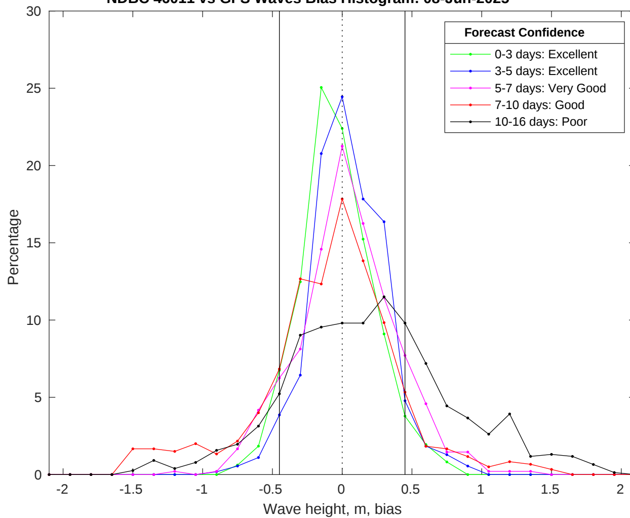
NDBC 46011 vs GFS Waves Bias Histogram: 08-Jun-2025
