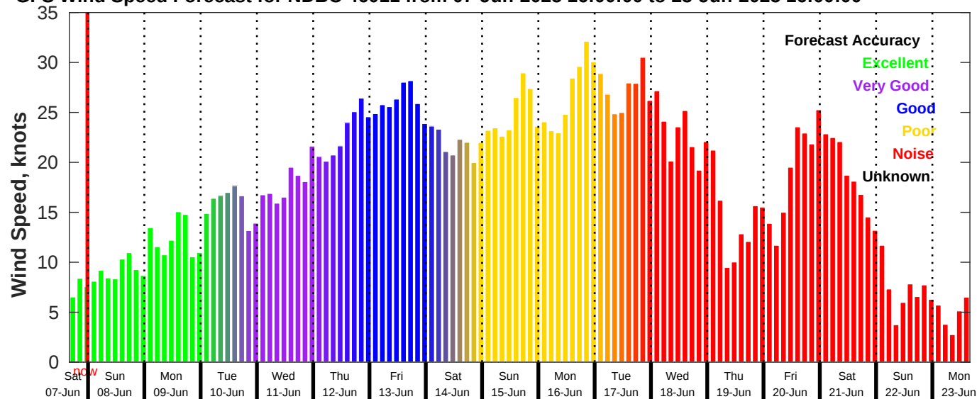
GFS Wind Speed Forecast for NDBC 46011 from 07-Jun-2025 16:00:00 to 23-Jun-2025 16:00:00
