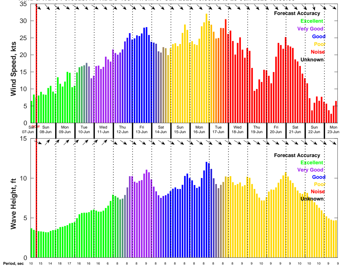
Wind & Wave Forecast for NDBC 46011 from 07-Jun-2025 16:00:00 to 23-Jun-2025 16:00:00
