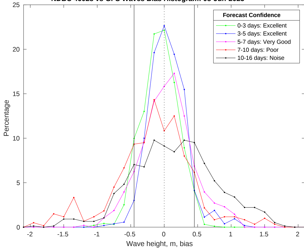
NDBC 46028 vs GFS Waves Bias Histogram: 08-Jun-2025
