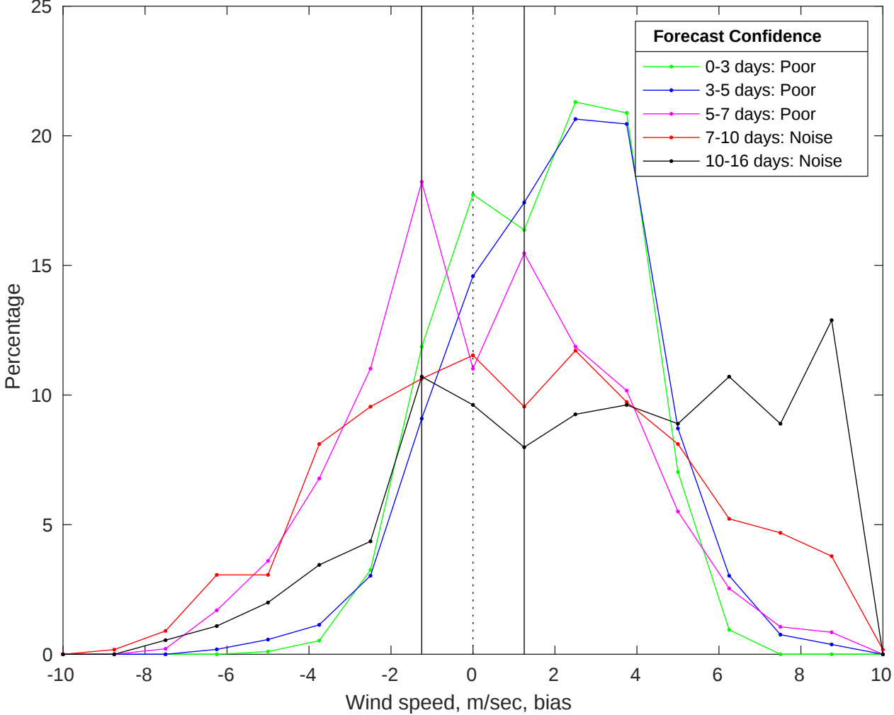
NDBC 46028 vs GFS Winds Bias Histogram: 08-Jun-2025
