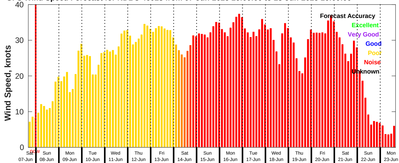
GFS Wind Speed Forecast for NDBC 46028 from 07-Jun-2025 16:00:00 to 23-Jun-2025 16:00:00
