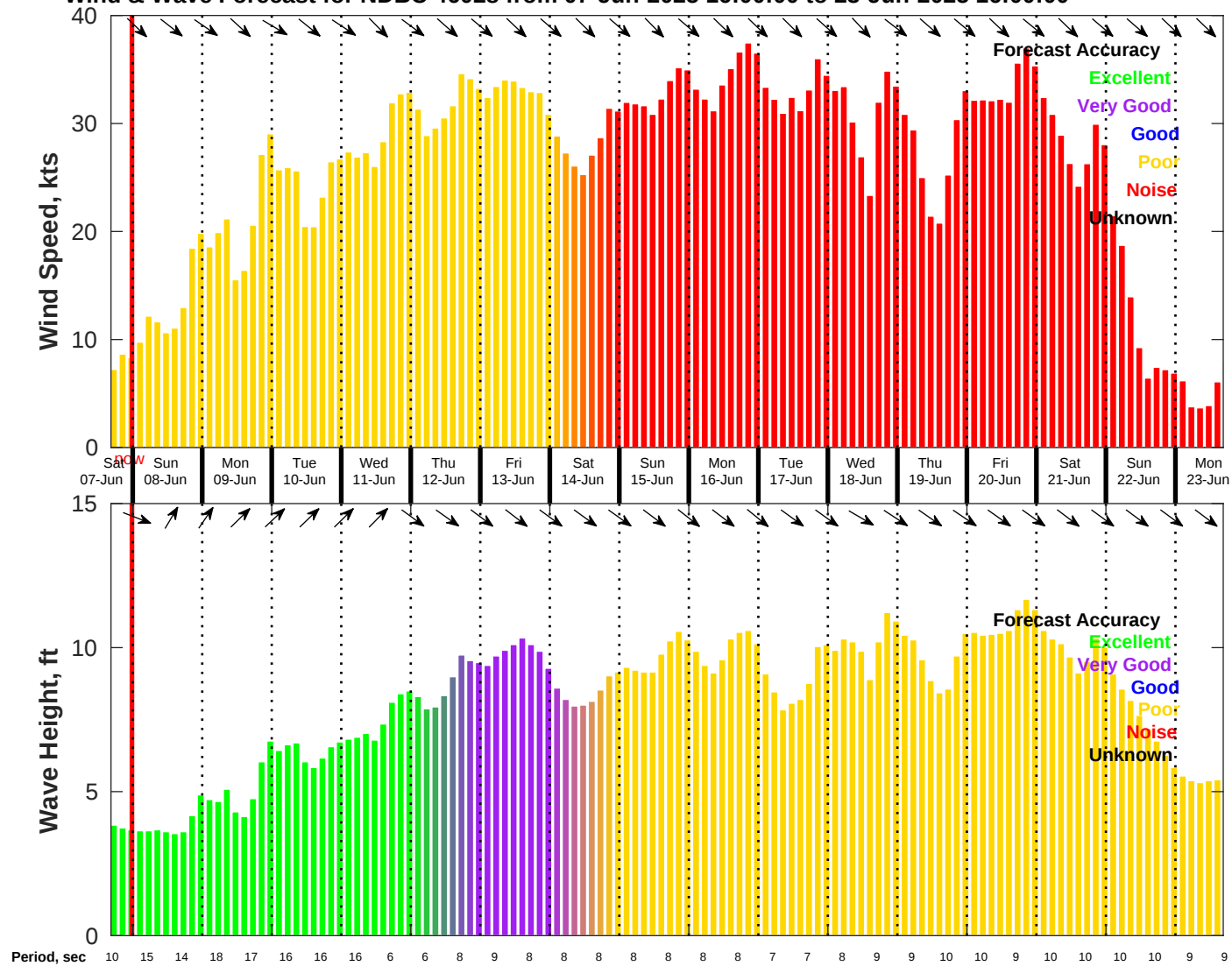
Wind & Wave Forecast for NDBC 46028 from 07-Jun-2025 16:00:00 to 23-Jun-2025 16:00:00
