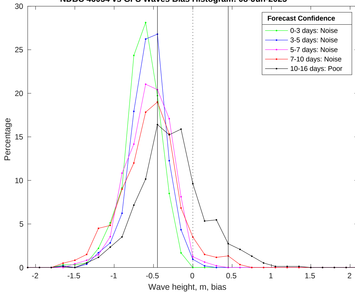
NDBC 46054 vs GFS Waves Bias Histogram: 08-Jun-2025
