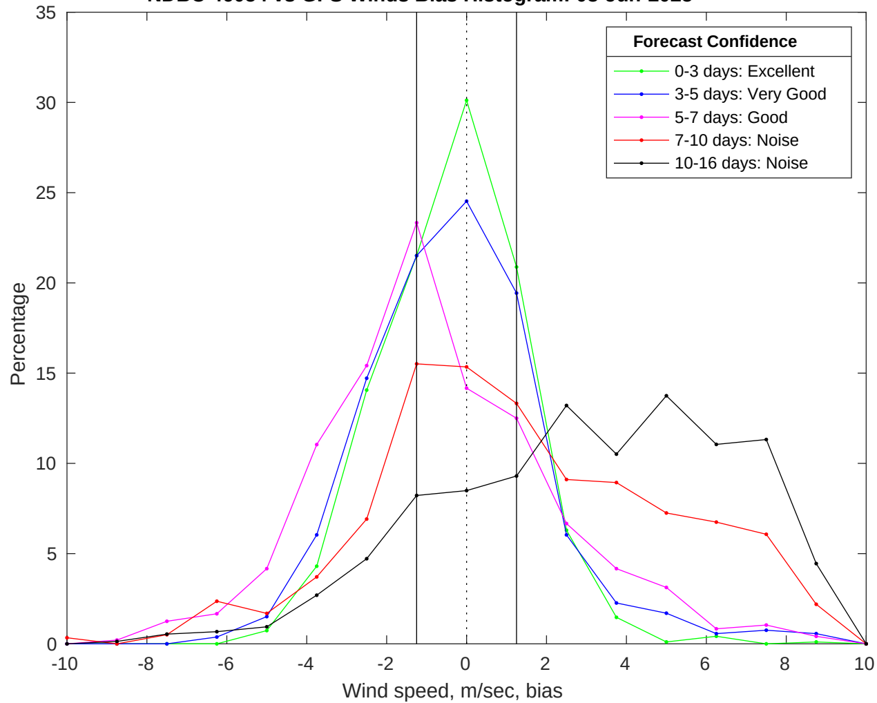
NDBC 46054 vs GFS Winds Bias Histogram: 08-Jun-2025
