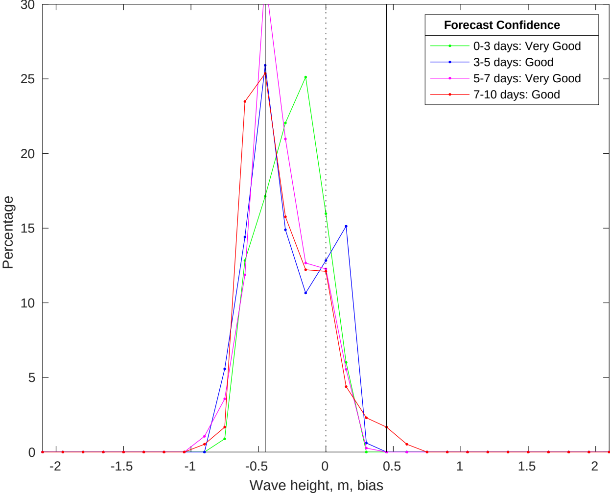
NDBC 51209 vs CMEMS Waves Bias Histogram: 08-Jun-2025
