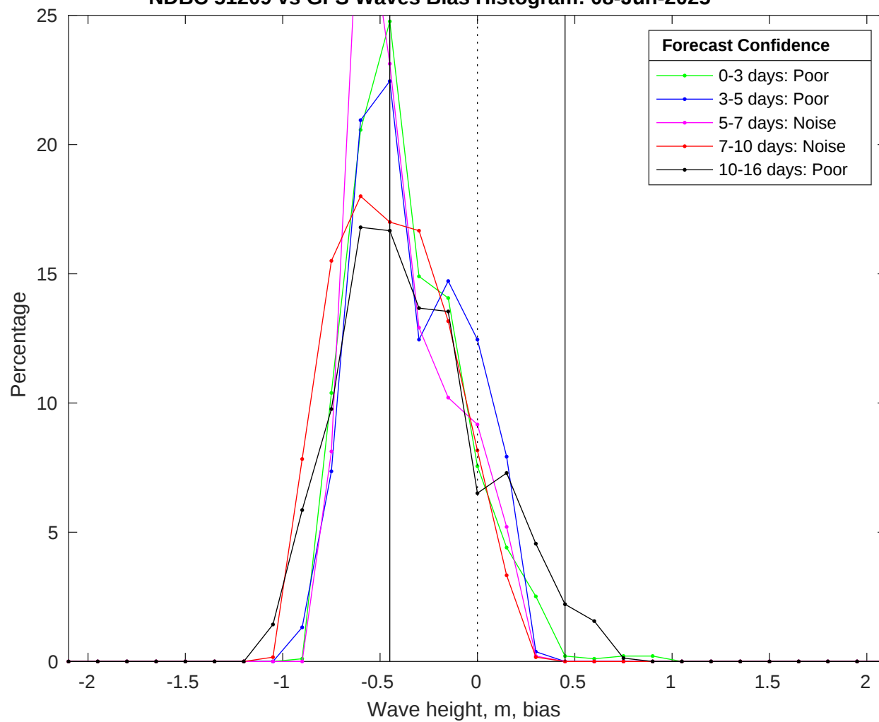
NDBC 51209 vs GFS Waves Bias Histogram: 08-Jun-2025
