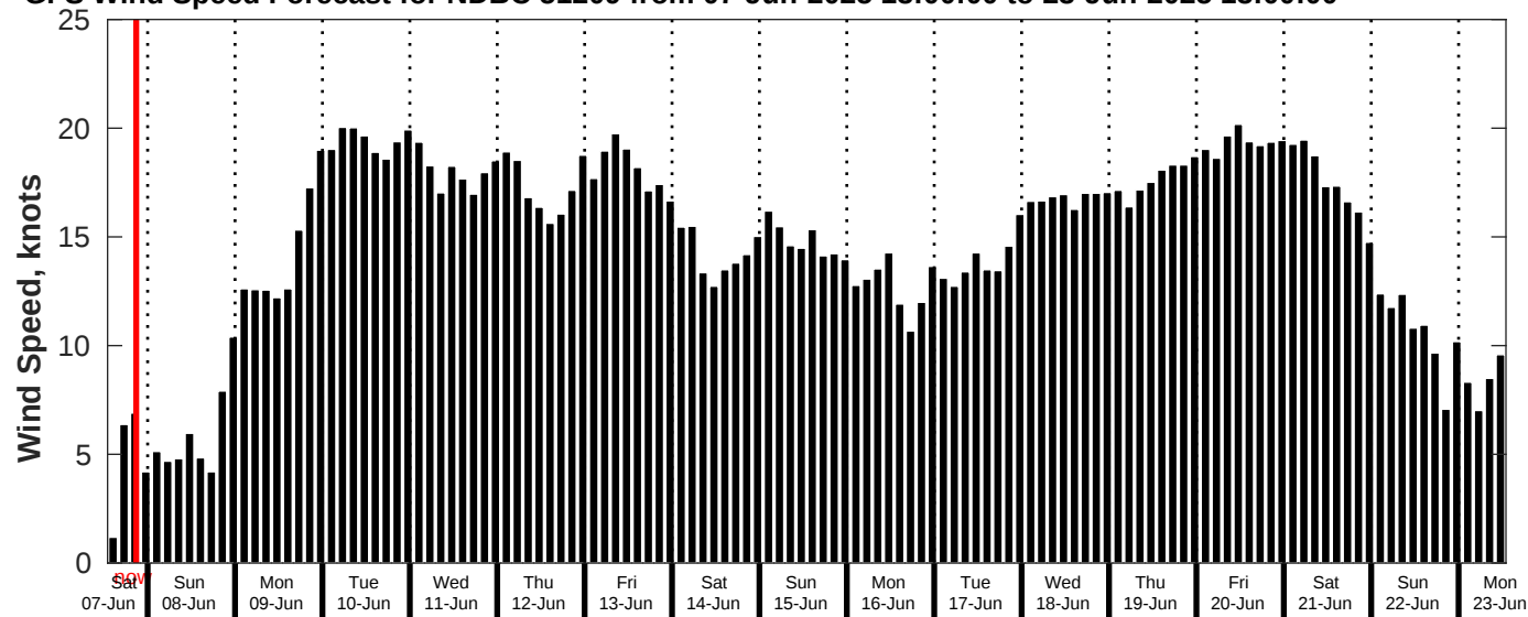
GFS Wind Speed Forecast for NDBC 51209 from 07-Jun-2025 13:00:00 to 23-Jun-2025 13:00:00
