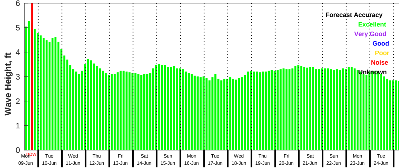
GFS Wave Forecast for NDBC 52211 from 08-Jun-2025 10:00:00 to 24-Jun-2025 10:00:00
