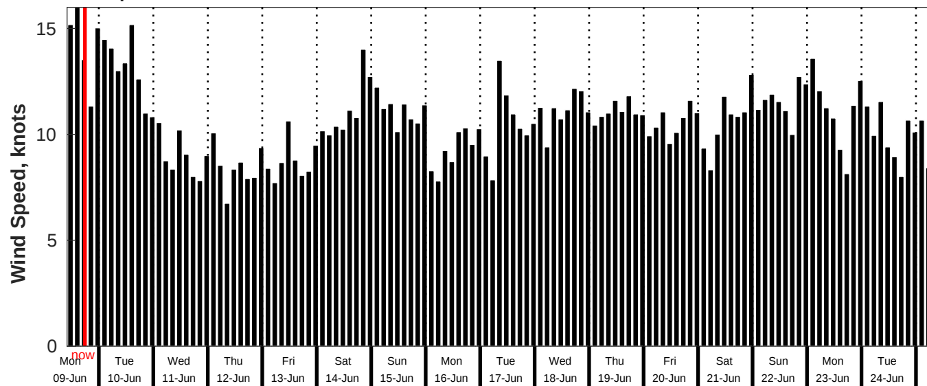
GFS Wind Speed Forecast for NDBC 52211 from 08-Jun-2025 10:00:00 to 24-Jun-2025 10:00:00
