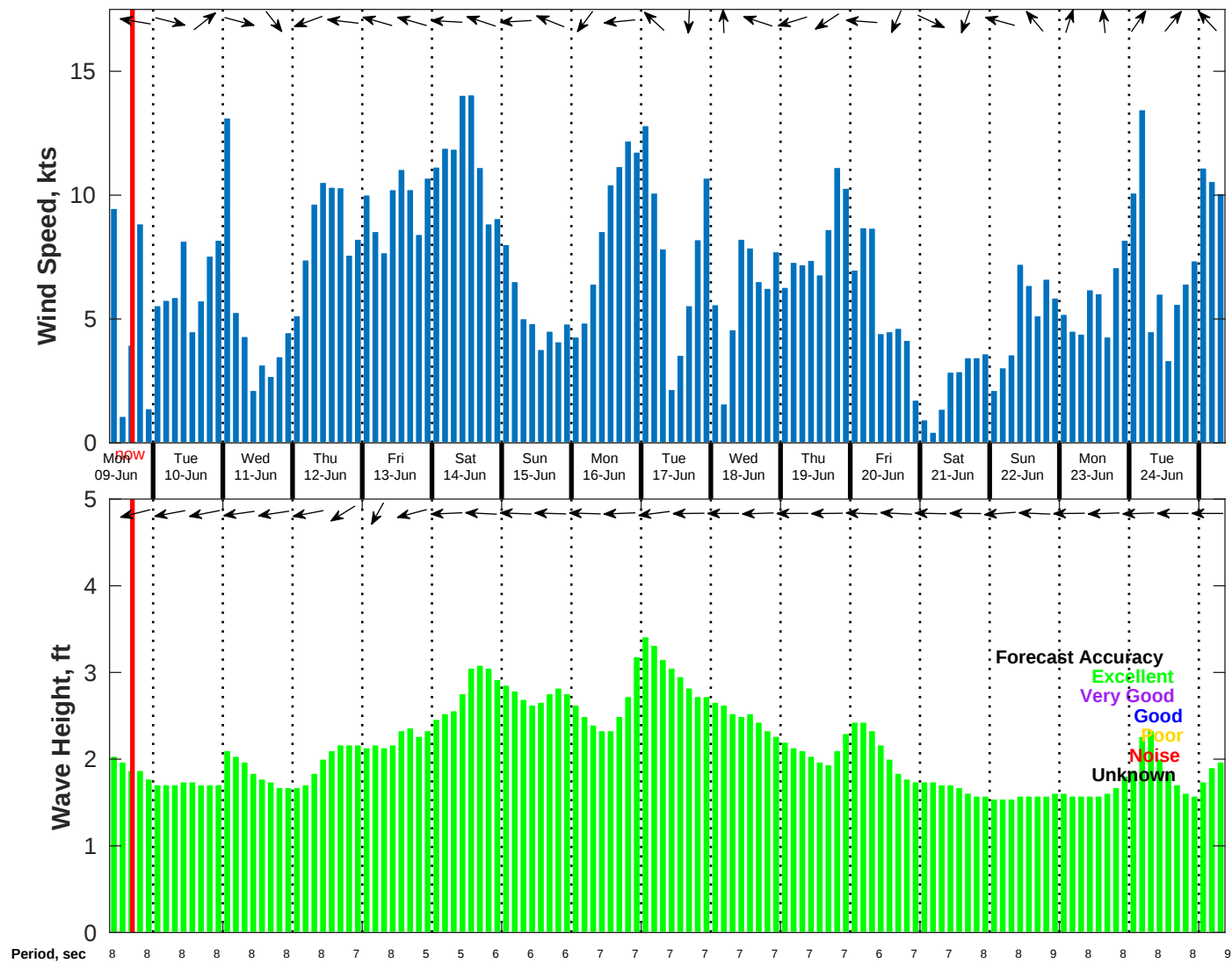
Wind & Wave Forecast for NDBC 52212 from 08-Jun-2025 09:00:00 to 24-Jun-2025 09:00:00
