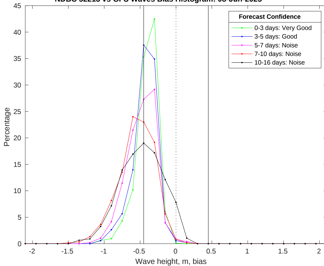
NDBC 52213 vs GFS Waves Bias Histogram: 08-Jun-2025
