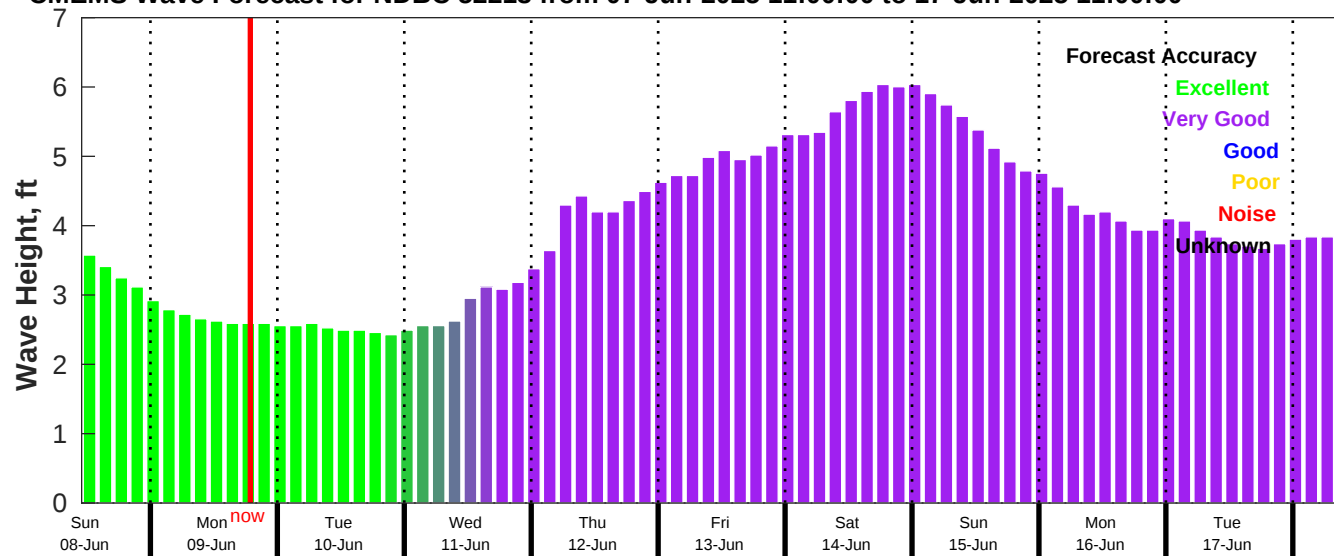
CMEMS Wave Forecast for NDBC 52213 from 07-Jun-2025 11:00:00 to 17-Jun-2025 11:00:00
