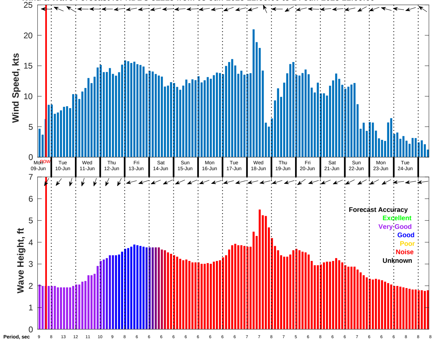
Wind & Wave Forecast for NDBC 52213 from 08-Jun-2025 11:00:00 to 24-Jun-2025 11:00:00
