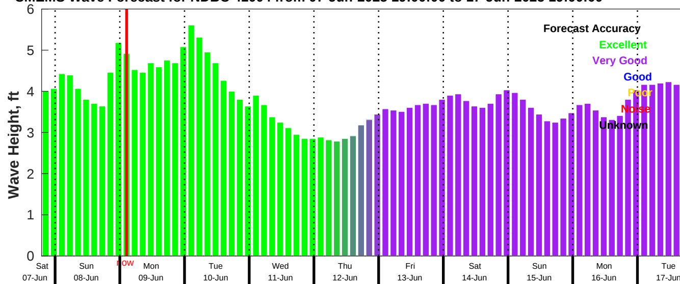
CMEMS Wave Forecast for NDBC 41004 from 07-Jun-2025 19:00:00 to 17-Jun-2025 19:00:00
