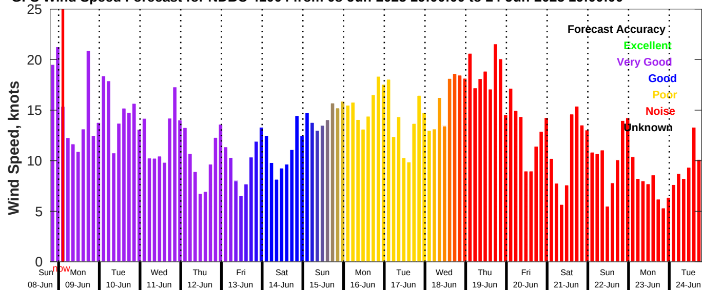
GFS Wind Speed Forecast for NDBC 41004 from 08-Jun-2025 19:00:00 to 24-Jun-2025 19:00:00
