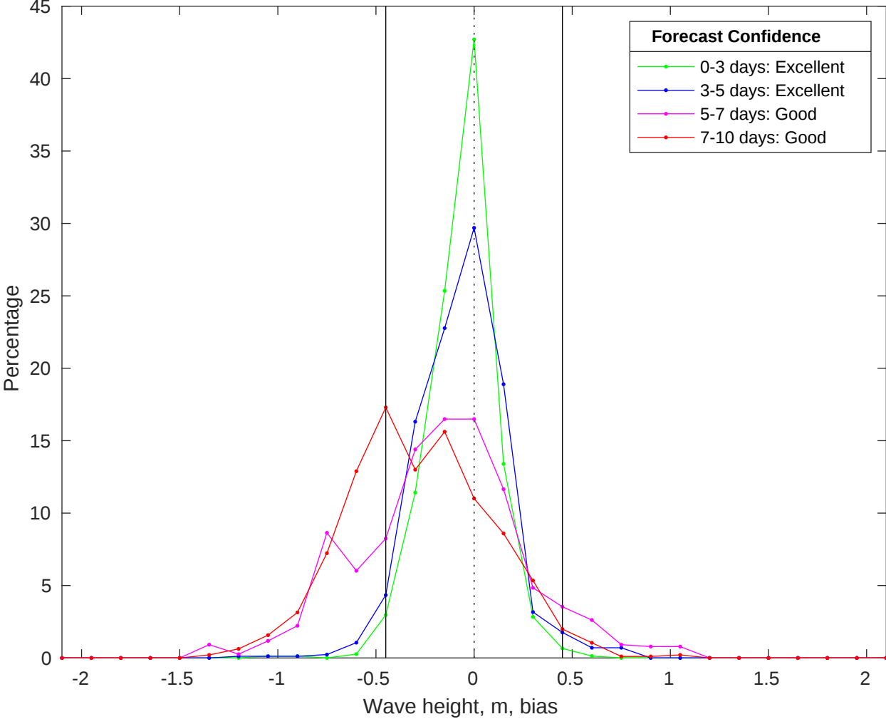
NDBC 41013 vs CMEMS Waves Bias Histogram: 09-Jun-2025
