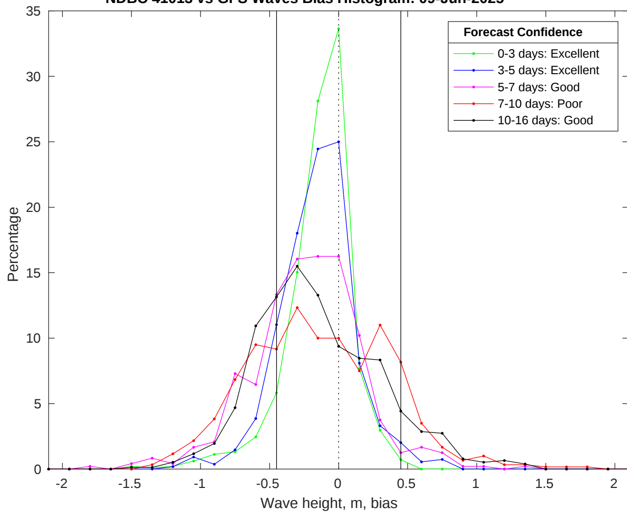
NDBC 41013 vs GFS Waves Bias Histogram: 09-Jun-2025
