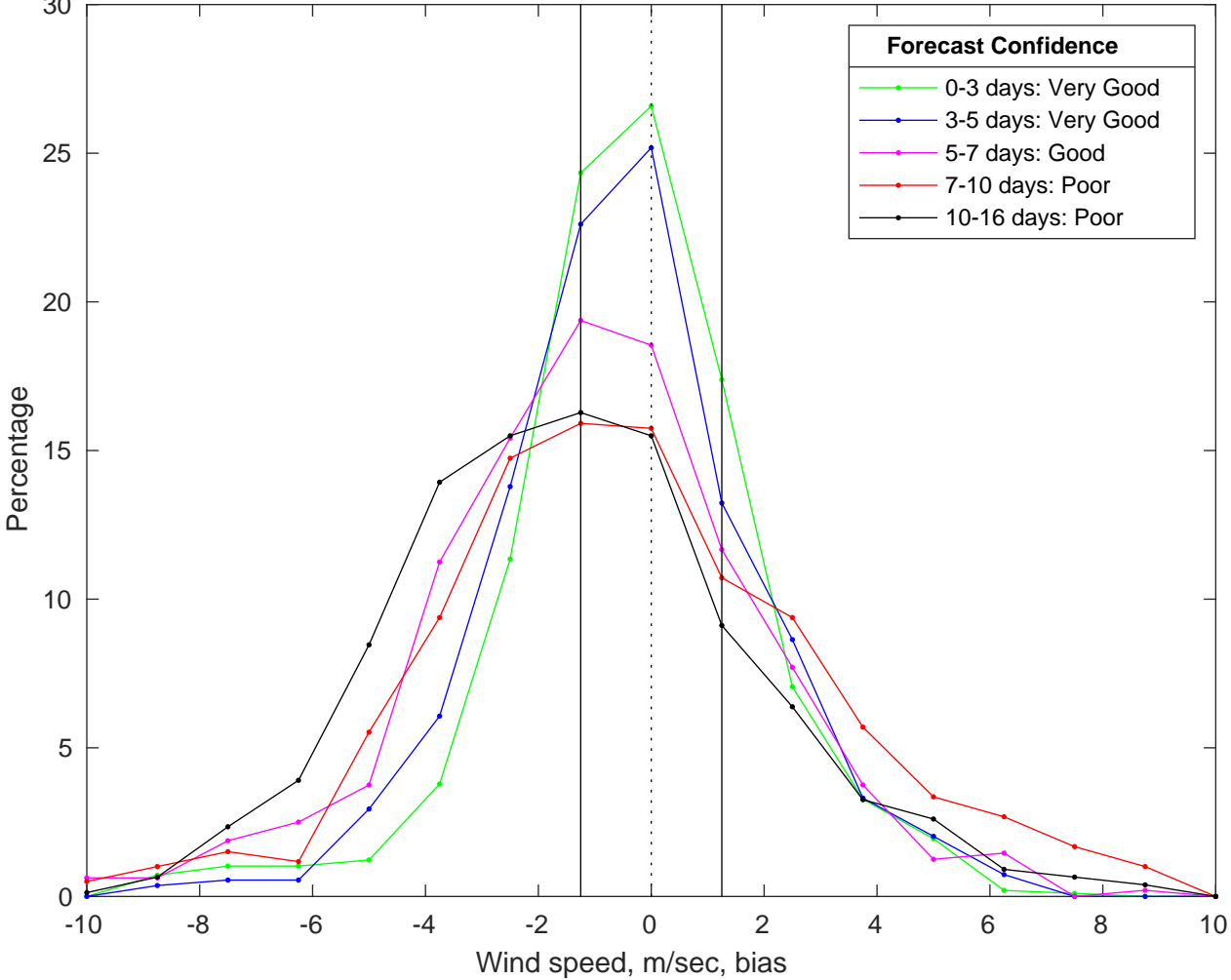
NDBC 41013 vs GFS Winds Bias Histogram: 09-Jun-2025
