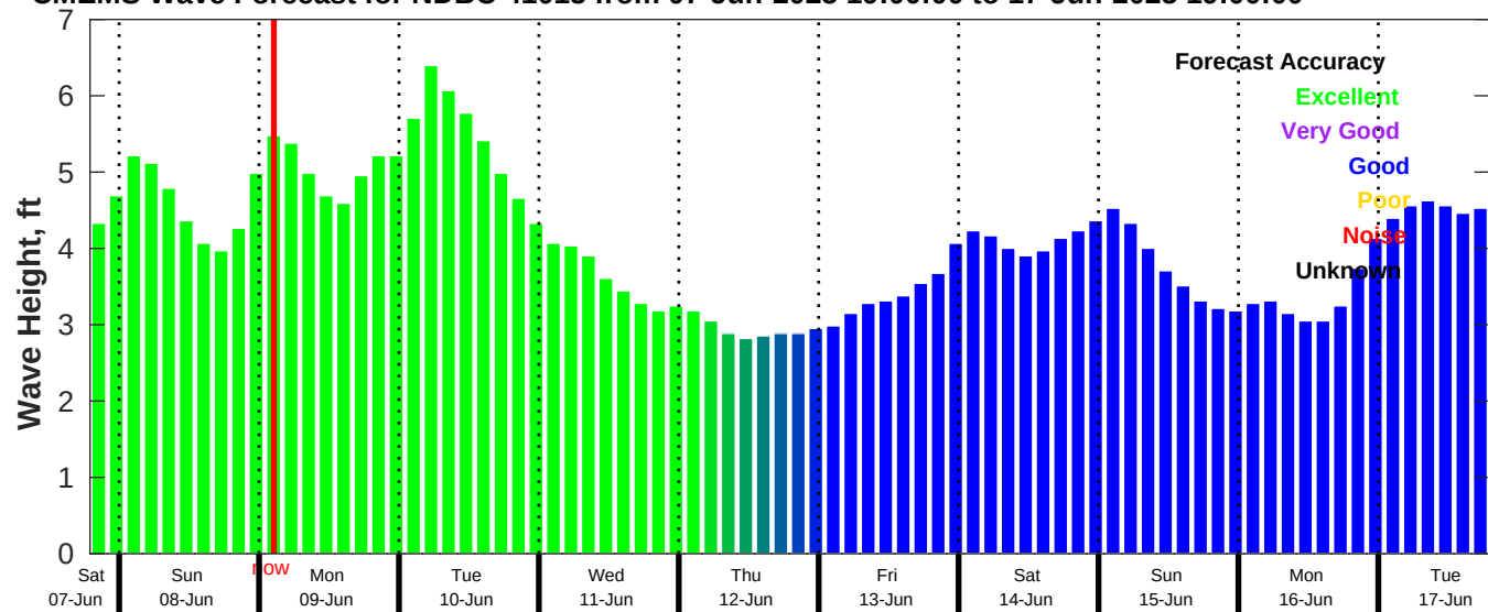
CMEMS Wave Forecast for NDBC 41013 from 07-Jun-2025 19:00:00 to 17-Jun-2025 19:00:00
