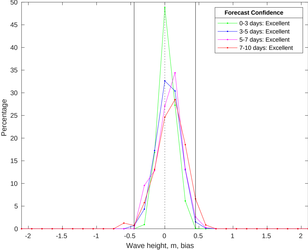
NDBC 41040 vs CMEMS Waves Bias Histogram: 09-Jun-2025
