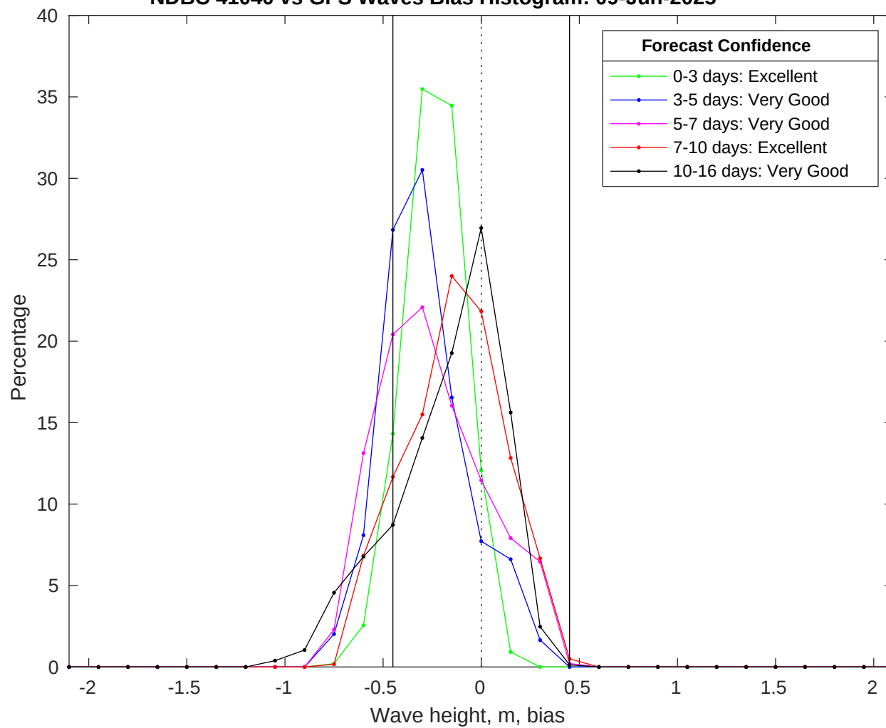
NDBC 41040 vs GFS Waves Bias Histogram: 09-Jun-2025
