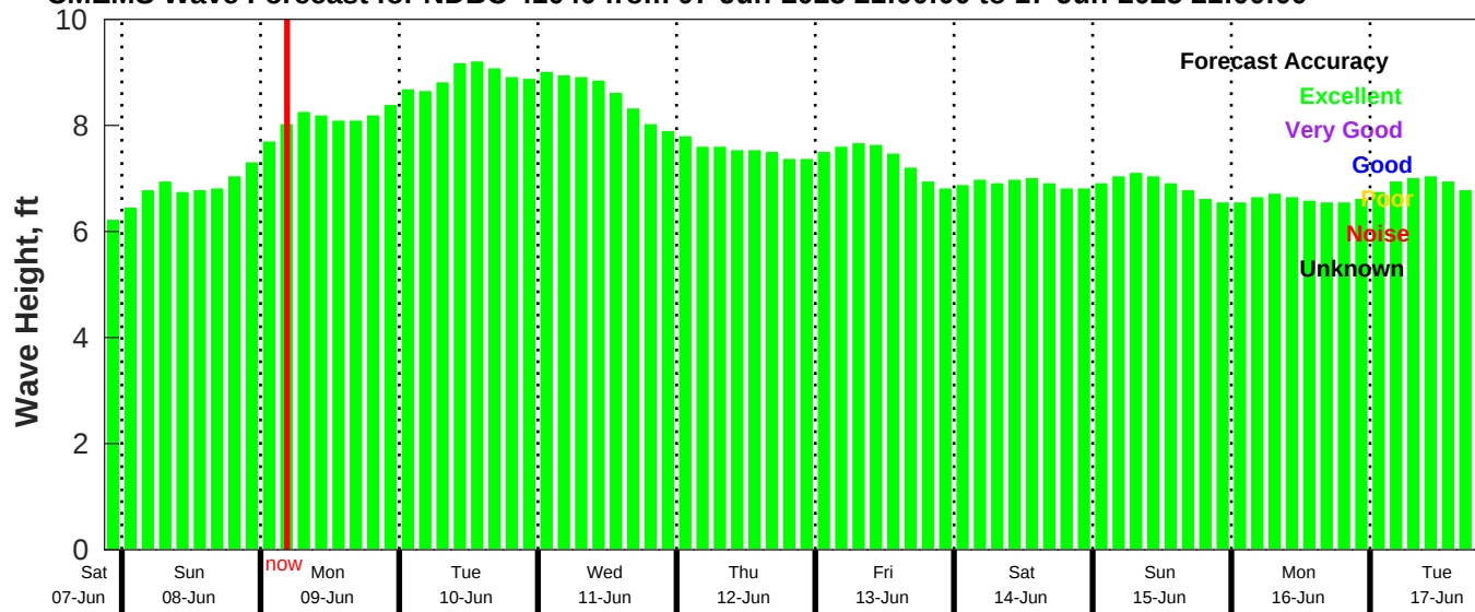
CMEMS Wave Forecast for NDBC 41040 from 07-Jun-2025 21:00:00 to 17-Jun-2025 21:00:00
