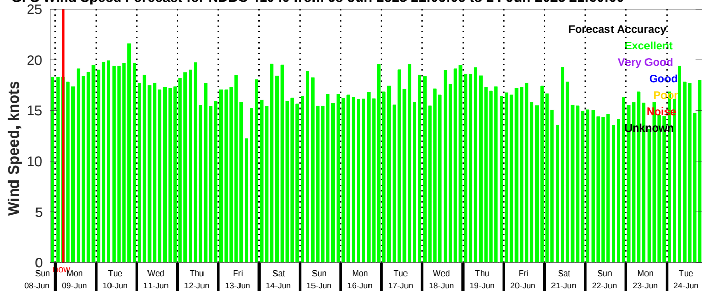
GFS Wind Speed Forecast for NDBC 41040 from 08-Jun-2025 21:00:00 to 24-Jun-2025 21:00:00
