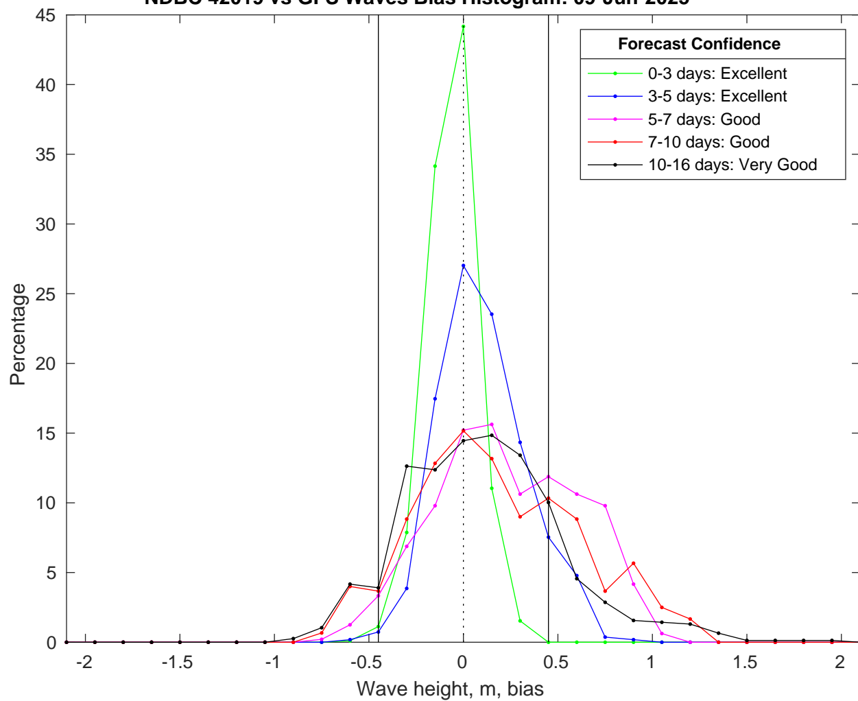
NDBC 42019 vs GFS Waves Bias Histogram: 09-Jun-2025
