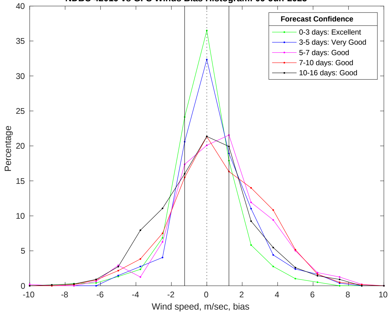
NDBC 42019 vs GFS Winds Bias Histogram: 09-Jun-2025
