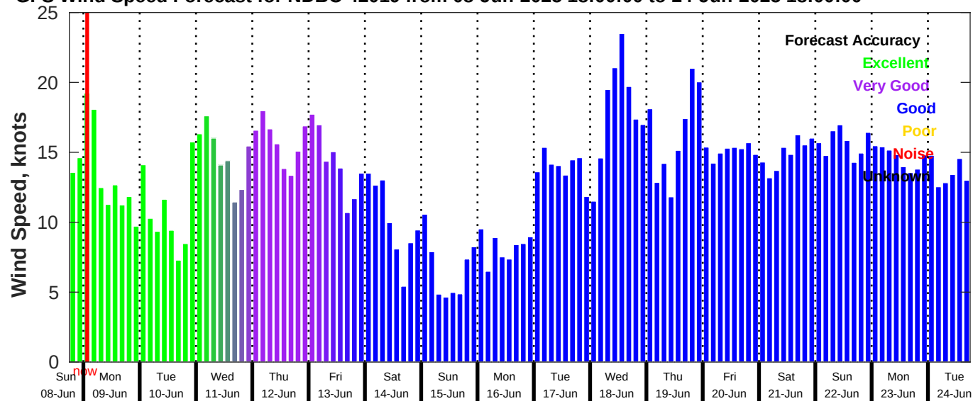
GFS Wind Speed Forecast for NDBC 42019 from 08-Jun-2025 18:00:00 to 24-Jun-2025 18:00:00
