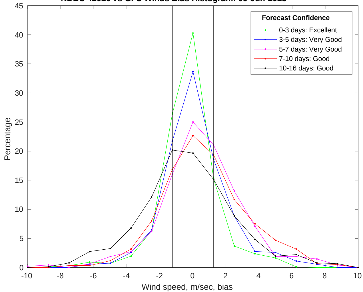
NDBC 42020 vs GFS Winds Bias Histogram: 09-Jun-2025
