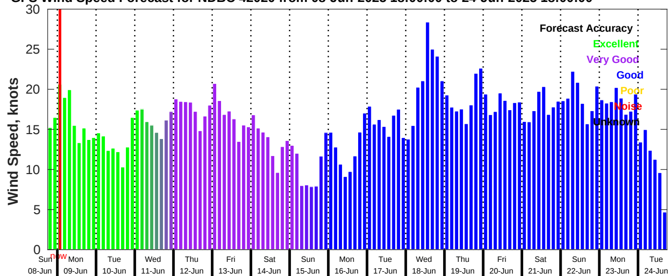
GFS Wind Speed Forecast for NDBC 42020 from 08-Jun-2025 18:00:00 to 24-Jun-2025 18:00:00
