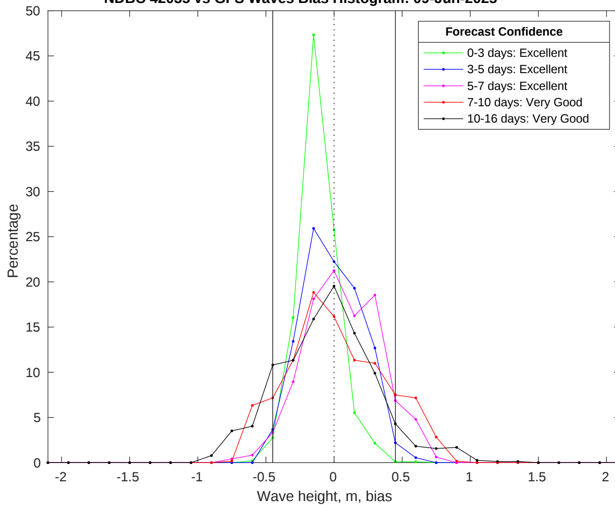
NDBC 42035 vs GFS Waves Bias Histogram: 09-Jun-2025
