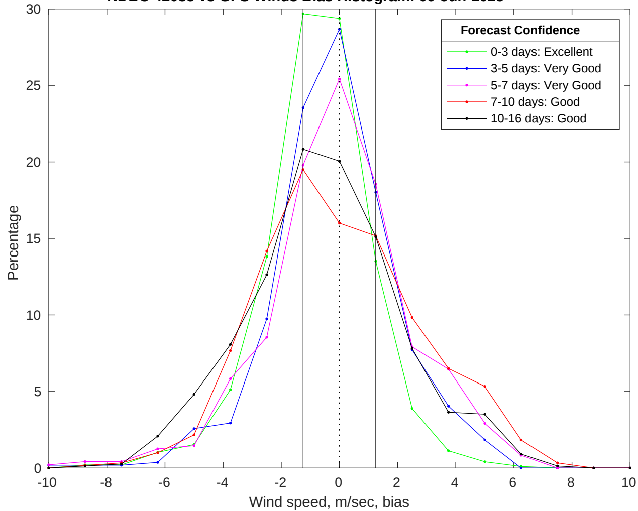
NDBC 42035 vs GFS Winds Bias Histogram: 09-Jun-2025
