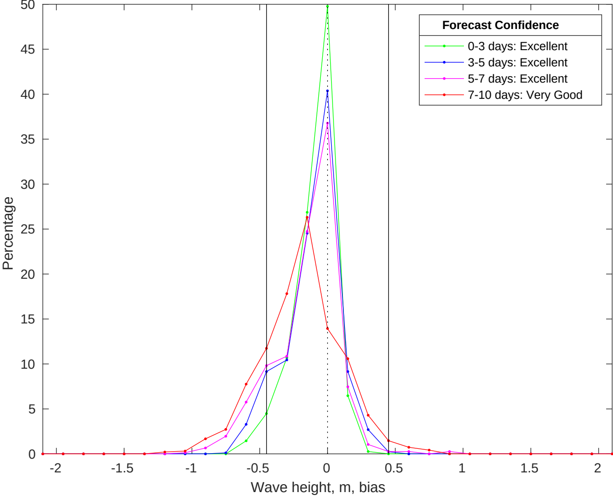
NDBC 42036 vs CMEMS Waves Bias Histogram: 09-Jun-2025
