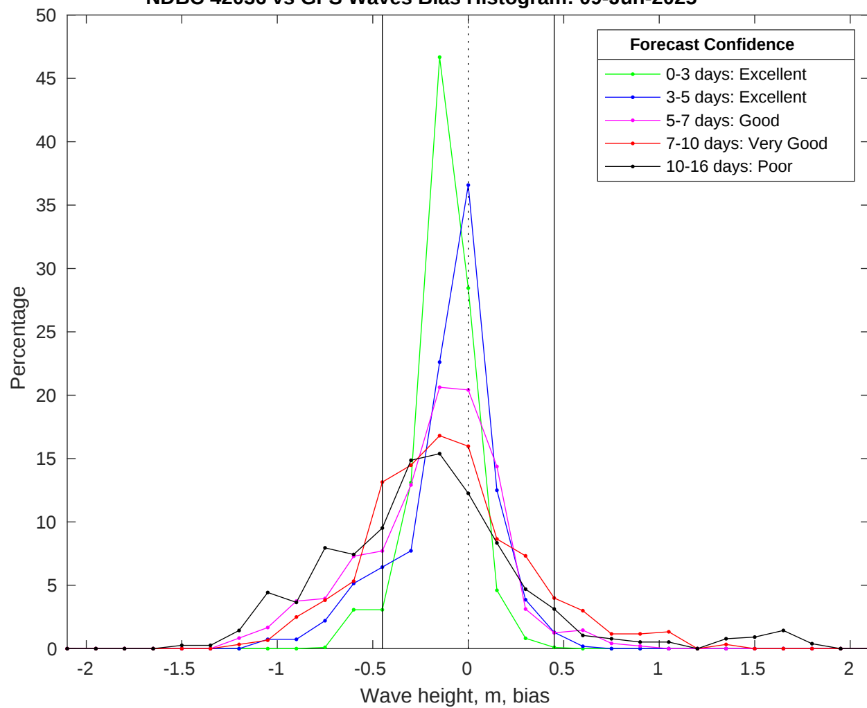
NDBC 42036 vs GFS Waves Bias Histogram: 09-Jun-2025
