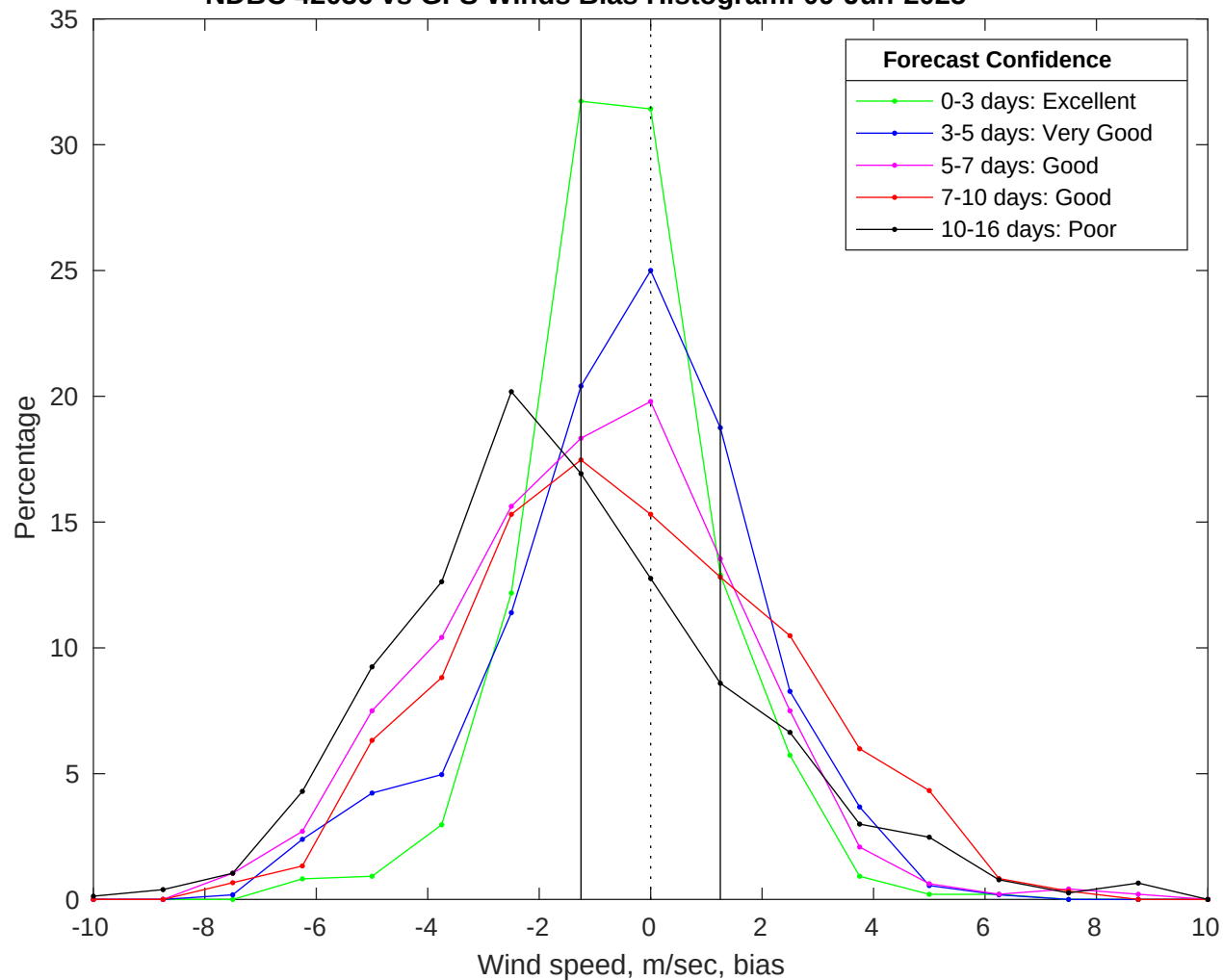
NDBC 42036 vs GFS Winds Bias Histogram: 09-Jun-2025
