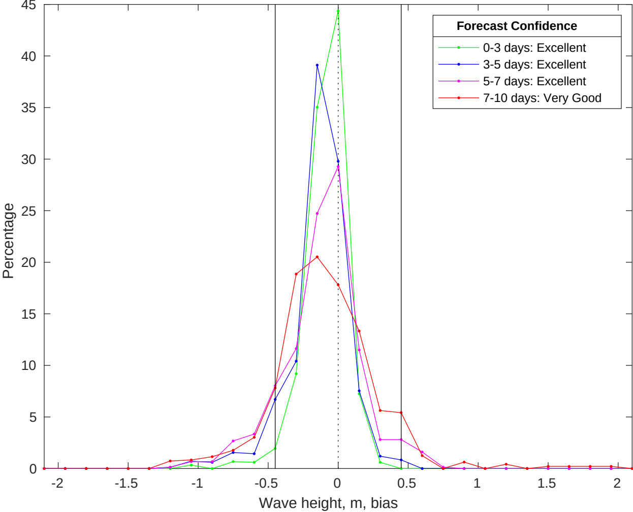
NDBC 42040 vs CMEMS Waves Bias Histogram: 09-Jun-2025
