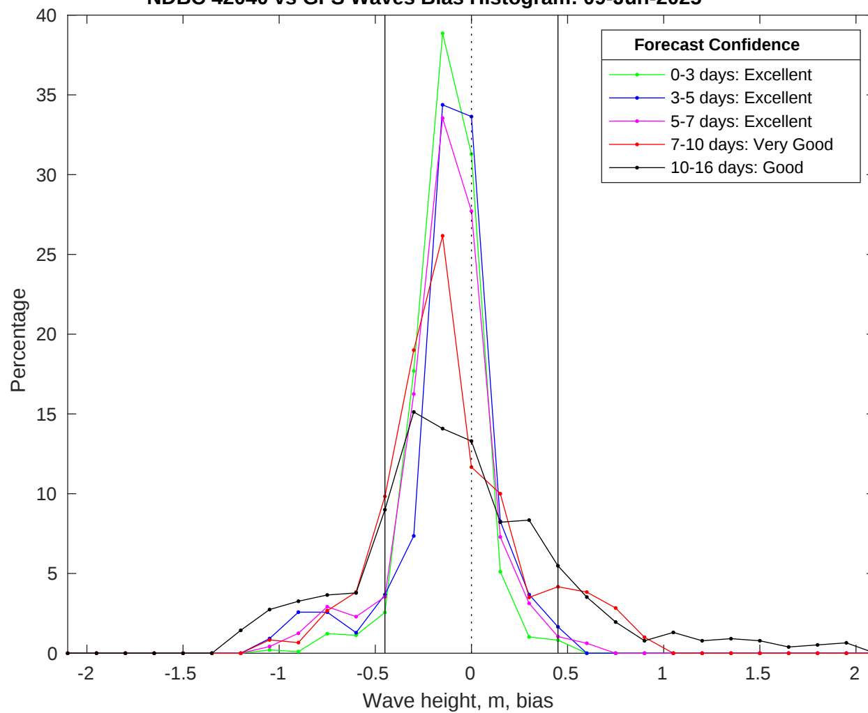
NDBC 42040 vs GFS Waves Bias Histogram: 09-Jun-2025
