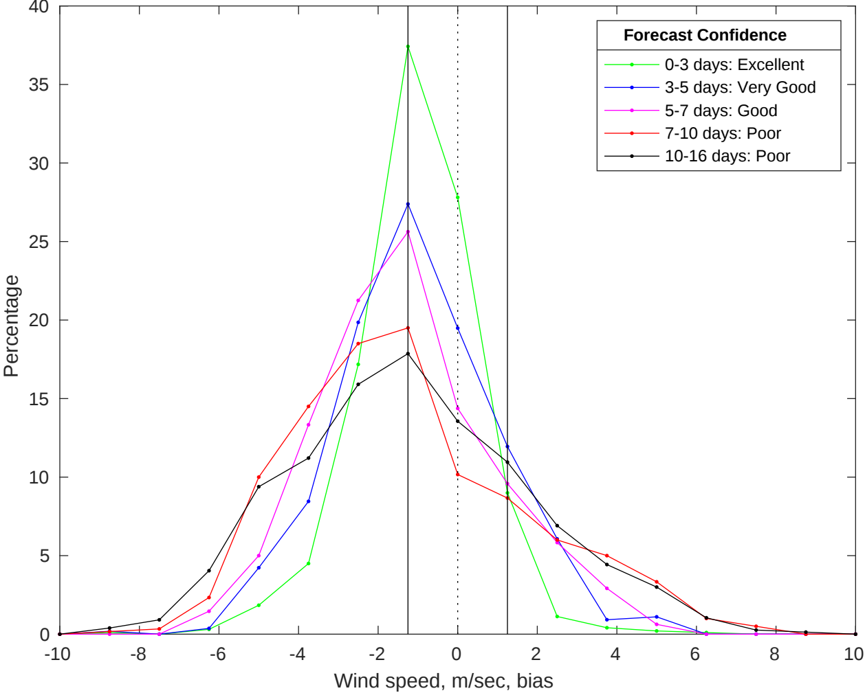
NDBC 42040 vs GFS Winds Bias Histogram: 09-Jun-2025
