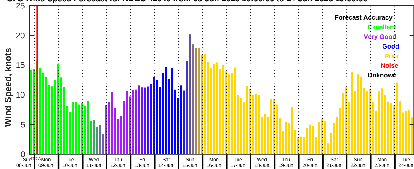
GFS Wind Speed Forecast for NDBC 42040 from 08-Jun-2025 19:00:00 to 24-Jun-2025 19:00:00
