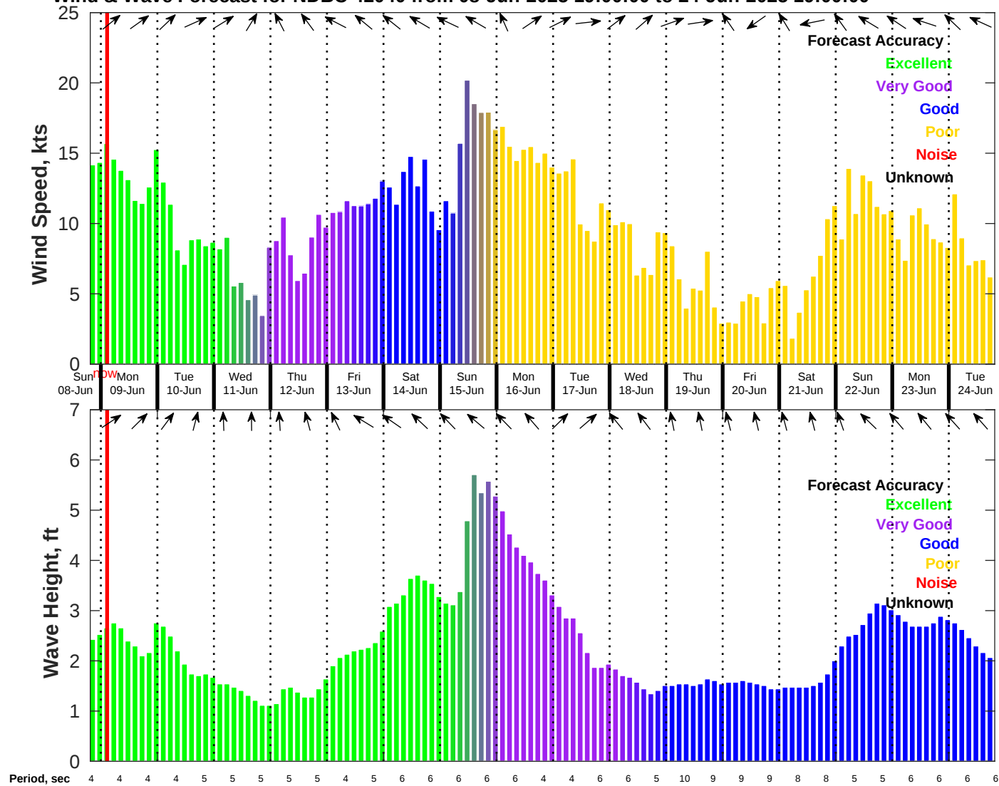
Wind & Wave Forecast for NDBC 42040 from 08-Jun-2025 19:00:00 to 24-Jun-2025 19:00:00
