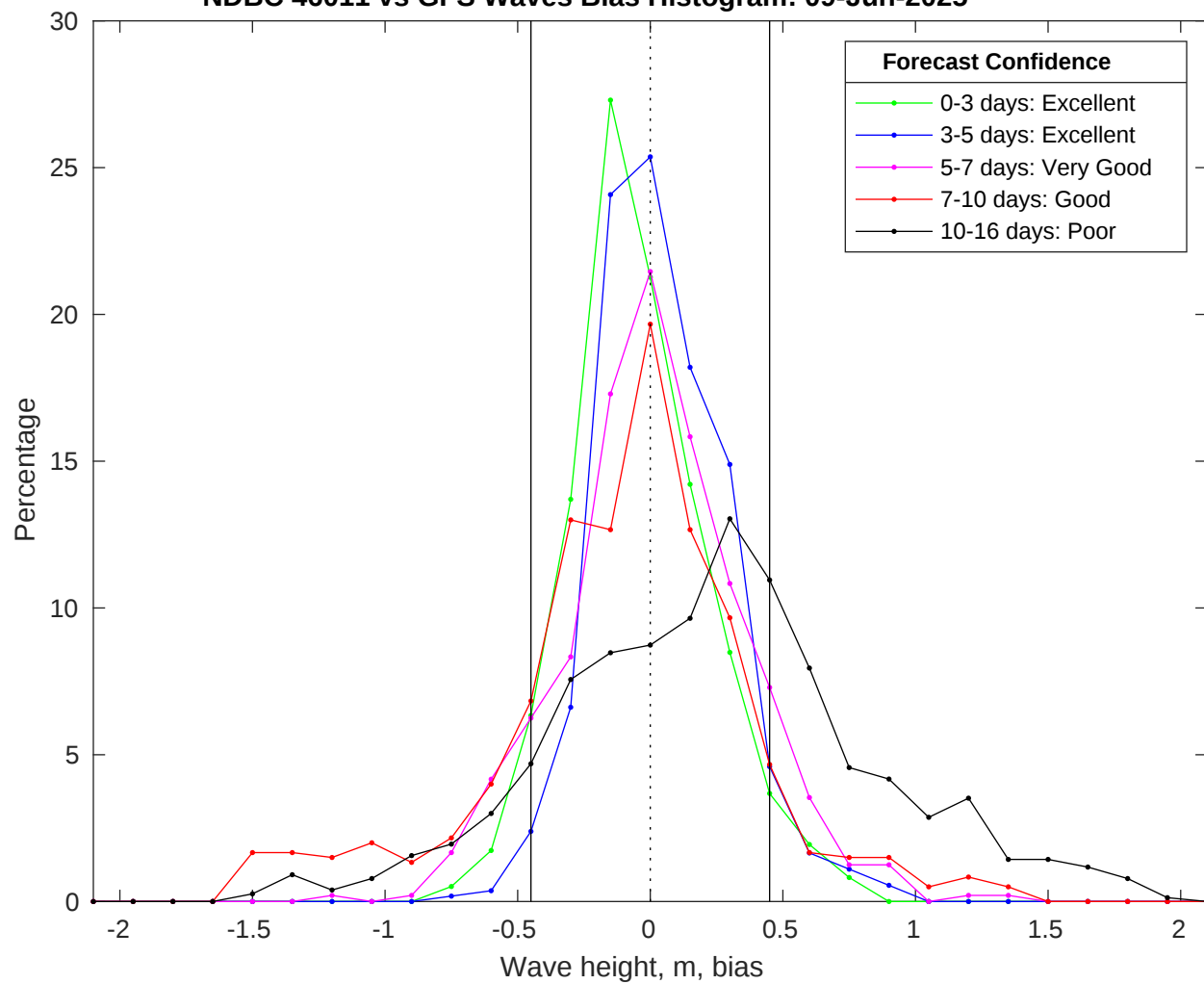
NDBC 46011 vs GFS Waves Bias Histogram: 09-Jun-2025
