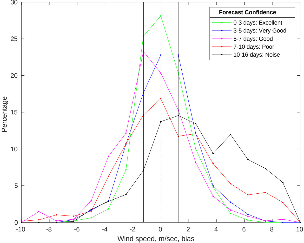
NDBC 46011 vs GFS Winds Bias Histogram: 09-Jun-2025
