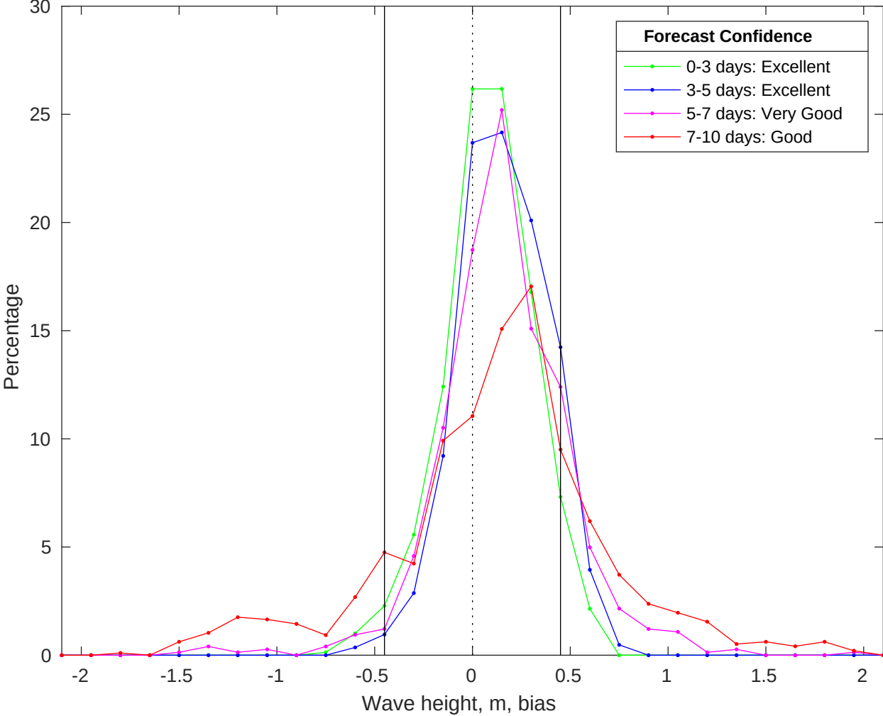
NDBC 46028 vs CMEMS Waves Bias Histogram: 09-Jun-2025
