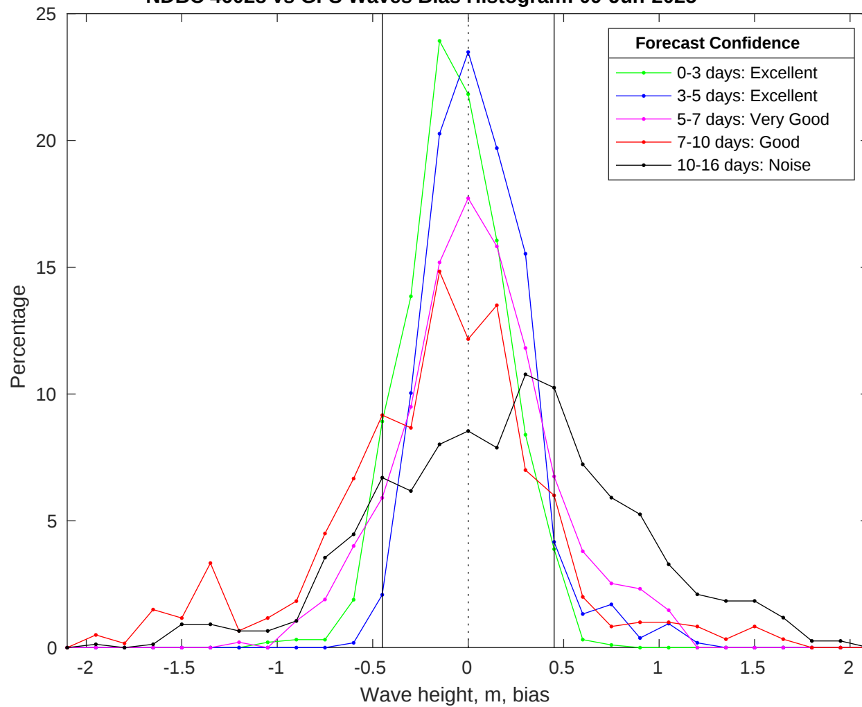
NDBC 46028 vs GFS Waves Bias Histogram: 09-Jun-2025
