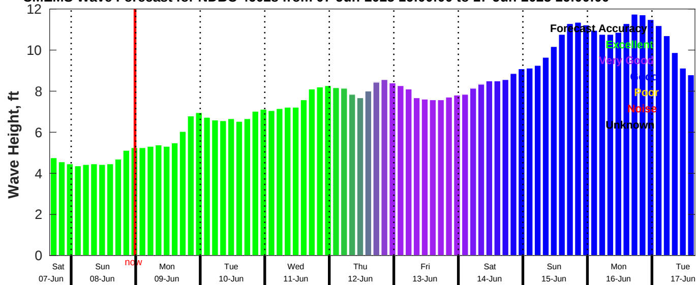
CMEMS Wave Forecast for NDBC 46028 from 07-Jun-2025 16:00:00 to 17-Jun-2025 16:00:00
